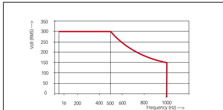
Voltage Vs frequency de-rating curve
