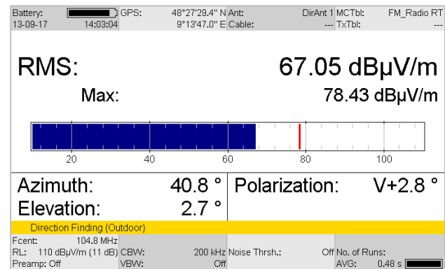
Direction finding using Manual Bearing
